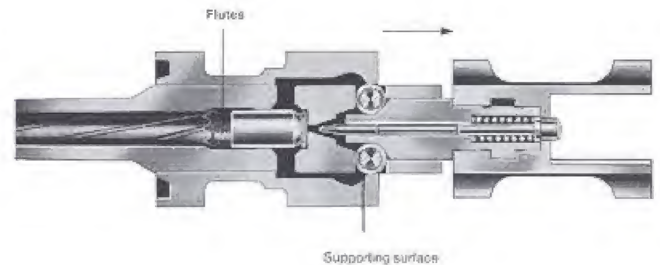
Fig. 28 Bolt in unlocked position
